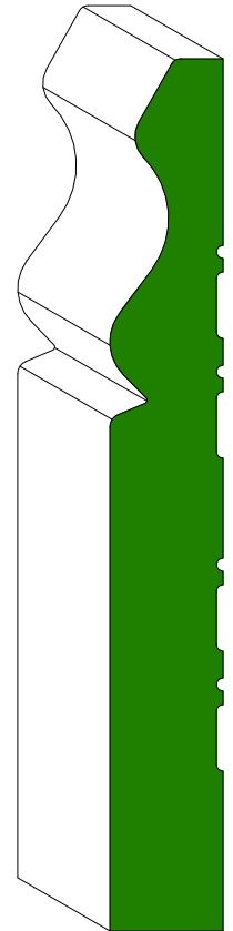
LRM WB 4 WOODARD 9/16 x 4-1/8 WF - Random FJ - 16'* PM - 16'*
