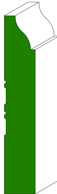
LRM 623 9/16 x 3-1/4 WF - Random PINE - Random FJ - 16* PM - 16* PT 623 MDF 16'
