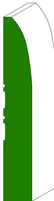
LRM 723 7/16 x 3-1/4 WF - Random PINE - Random FJ - Random
